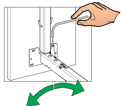
Angle adjustment.
